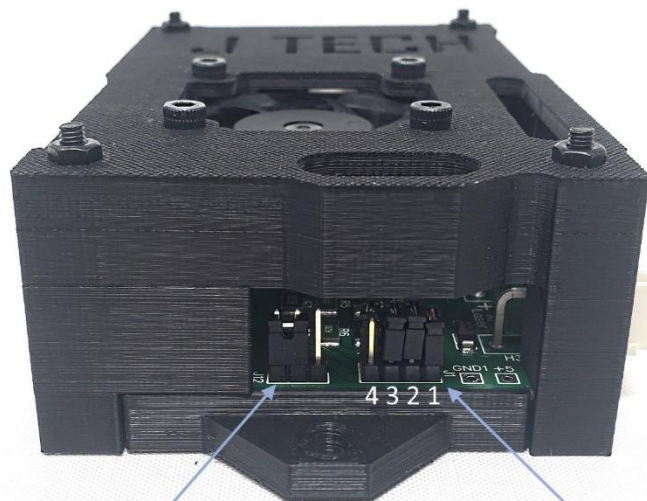
Jumper J1
