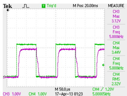
Typical Control Signal with "non inverting" set running at 3KHz. Ch 1 control, Ch 3 output.
